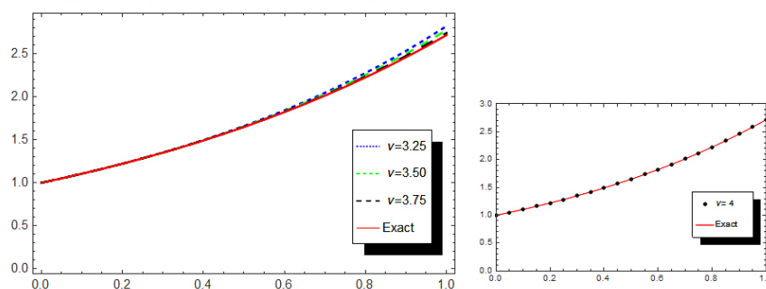
FIGURE 2. Comparison of y(x) for m = 3 , with \nu = 3.25, 3.50, 3.75, 4 and the exact solution for Example 6.1.
