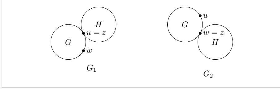
FIGURE 2. The transformation of two graphs.
