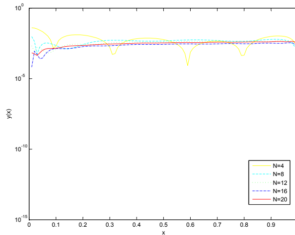
FIGURE 2. Error between the exact- and numerical- solutions of our method with g(x) = x^{0.5} for Example 5.5.
