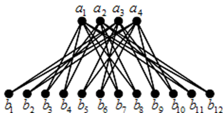
FIGURE 5. A balanced d-magic graph K_{1,3} \oplus K_{2,2} with 16 vertices and 24 edges.
