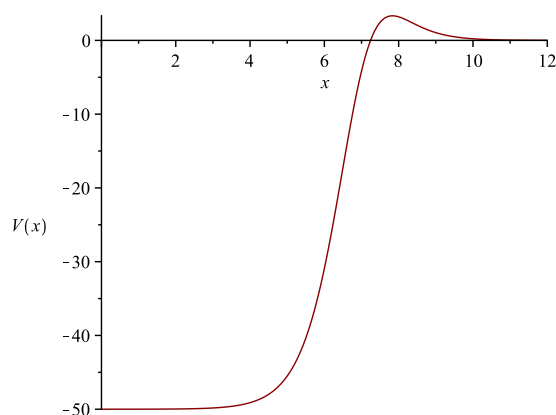
FIGURE 4. The Woods - Saxon potential.
