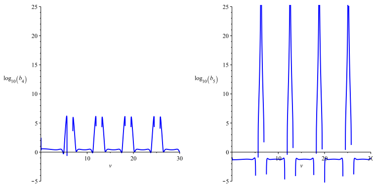
FIGURE 3. Behavior of the coefficients b_4 and b_5 of the new method.
