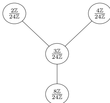
The graph of G^*(M) .
