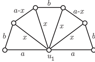
FIGURE 4. A typical magic labeling of F_7 .
