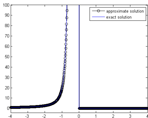
FIGURE 10. Comparison the approximate solution obtained by \delta -ziti's scheme with the exact solution in presence a singularity.
